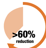
Hydrocarbons (HC)
