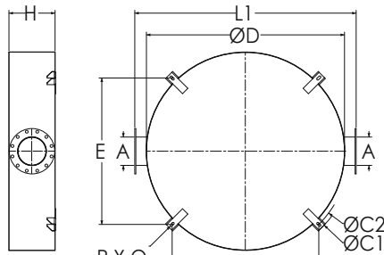
END IN END OUT (EI-EO)
