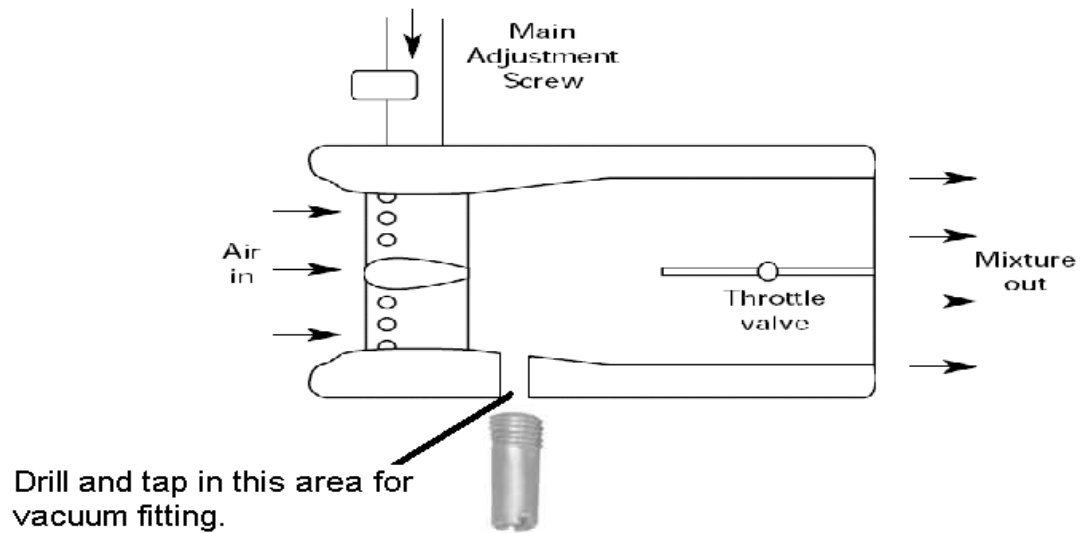
Fig 4a: Generic Fixed Venturi Vacuum Location
