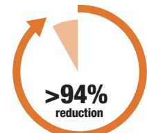
Hydrocarbons (HC)
